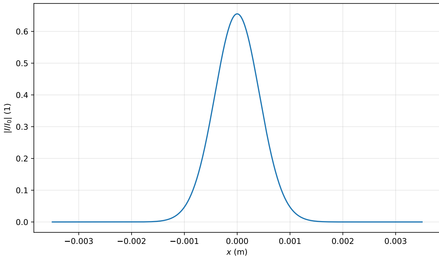
Intensity profile I(x, y = 0, z = 1.592m)/I_0 , P_{in}=0.1P_{cr} , artificial time
